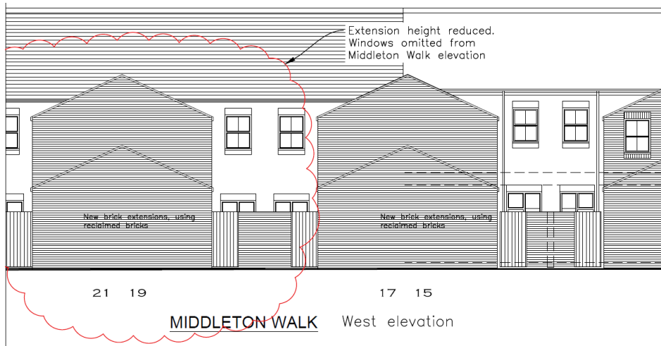
In-fill rear elevation showing roof height reduced by 0.5 m
